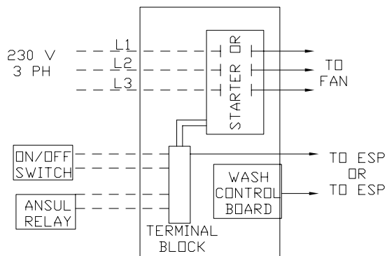
FIELD WIRING TO CONTROL PANEL
