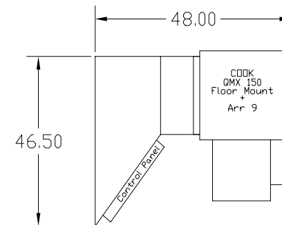
PLAN VIEW OF STANDARD FAN
