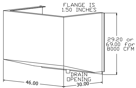
VERTICAL AIR INLET WITH DRAIN
