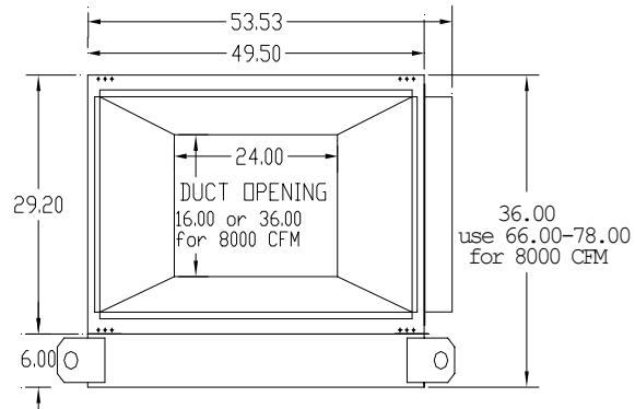
STANDARD HORIZONTAL AIR INLET
