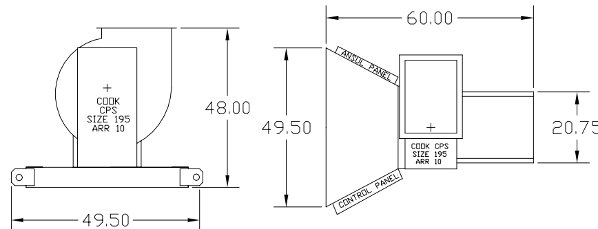
OPTIONAL OUTDOOR UPBLAST FAN with PLAN VIEW
